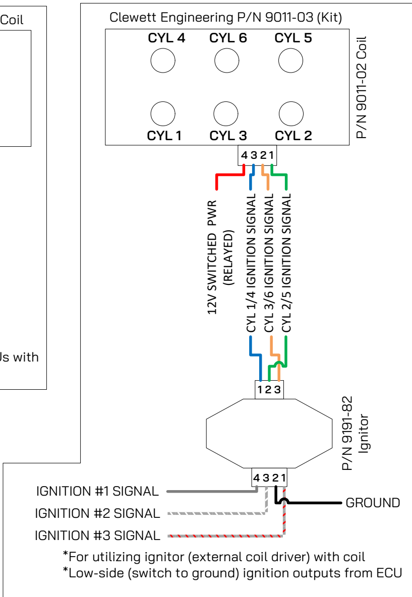
Bosch 3x2 Coil (Clewett Engineering 9011-02)
